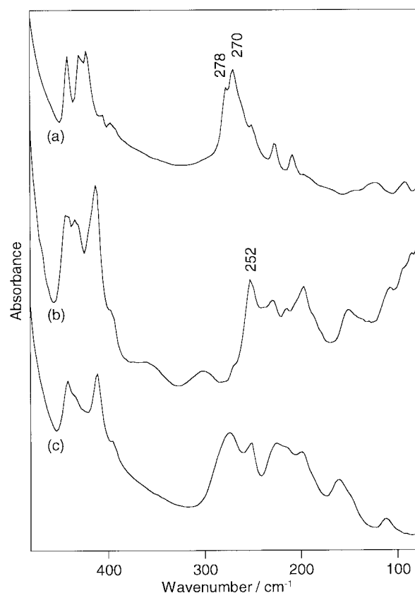
Fig. 3 Far-IR spectra of (a) [Cu(PPh 3 ) 2 O 2 CH], (b) [Cu(PPh 3 ) 3 O 2 CH]·0.5EtOH, and (c) [Cu(PPh 3 ) 3 O 2 CH]·HCO 2 H.
