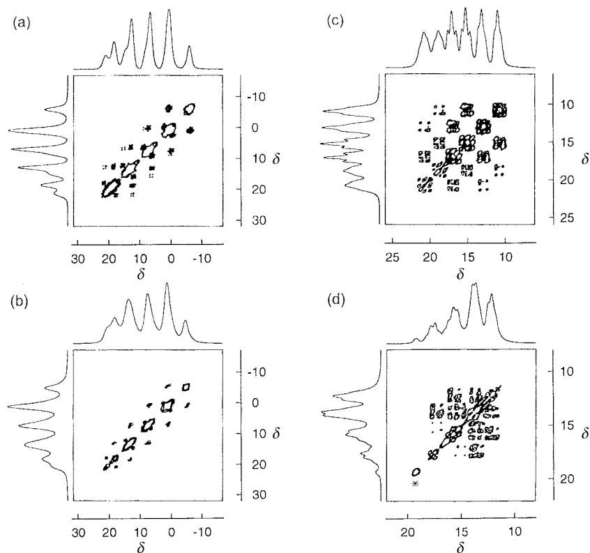
Fig. 6 Solid-state 2D ^{31}\text{P} CP COSY spectra of (a) [\text{Cu}(\text{PPh}_3)_3\text{O}_2\text{CH}]\cdot\text{HCO}_2\text{H} (b) [\text{Cu}(\text{PPh}_3)_3\text{O}_2\text{CH}]\cdot 0.5\text{EtOH} , (c) [\text{Ag}(\text{PPh}_3)_3\text{O}_2\text{CH}]\cdot\text{HCO}_2\text{H} and (d) [\text{Ag}(\text{PPh}_3)_3\text{O}_2\text{CH}] . Chemical shifts relative to solid \text{PPh}_3 . The resonance in (d) marked with an asterisk is due to an impurity.
