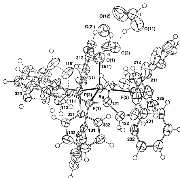
Fig. 1 Molecular structure of [\text{Ag}(\text{PPh}_3)_3\text{O}_2\text{CH}] \cdot \text{HCO}_2\text{H} (153 K determination) showing all non-hydrogen atoms and the atom numbering scheme, inclusive of disordered components excepting those for the minor components of the solvate molecule. 50% probability amplitude displacement ellipsoids are shown for the non-hydrogen atoms, hydrogen atoms having arbitrary radii of 0.1 Å.
